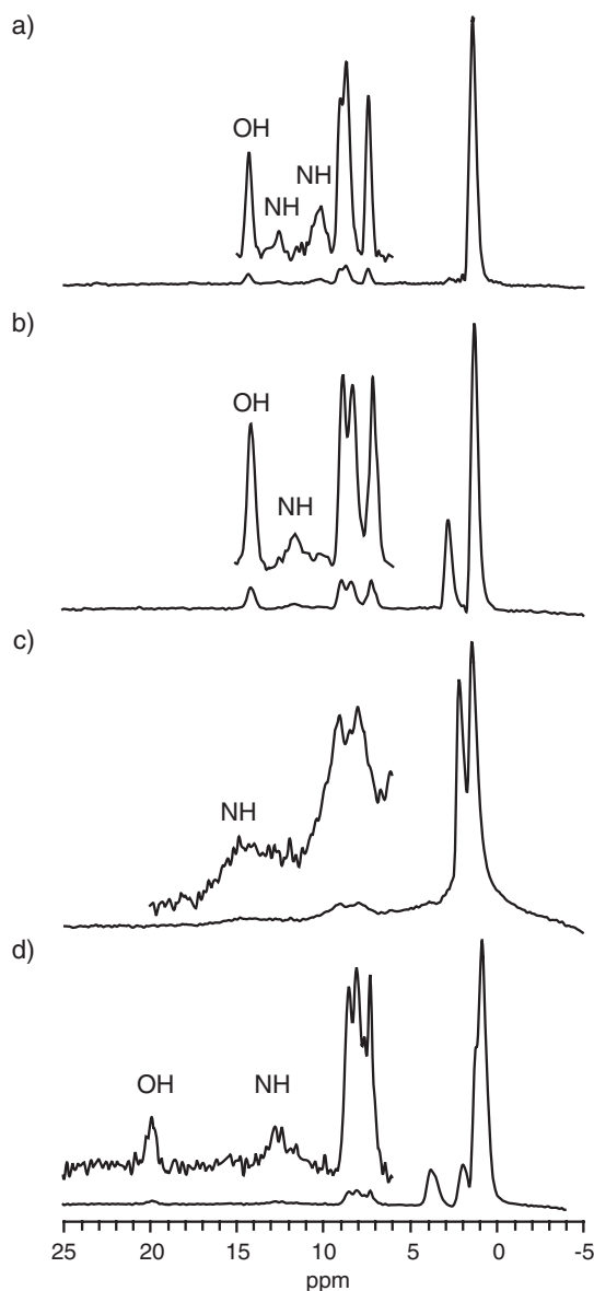
Fig. 2. 1 H NMR CRAMPS spectra of a) 2,6-( t -BuCONH) 2 C 6 H 3 COOH ( 1 ), b) 2- t -BuCONH-6-MeC 6 H 3 COOH ( 2 ), c) [NEt 4 ][2,6-( t -BuCONH) 2 C 6 H 3 COO] ( 3 ), and d) [N( n -Pr) 4 ][H{2,6-( t -BuCONH) 2 C 6 H 3 (COO)} 2 ] ( 4 ) in the solid state.
