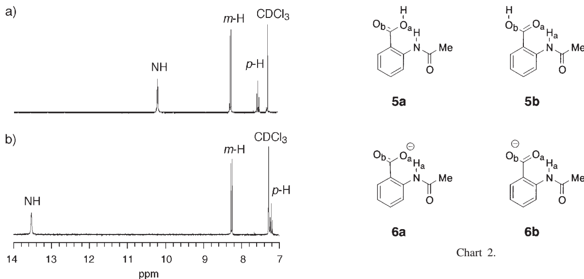
Fig. 3. ^1\text{H} NMR spectra of a) 2,6-( t -BuCONH) _2 C _6 H _3 -COOH ( 1 ) and b) [NEt _4 ][2,6-( t -BuCONH) _2 C _6 H _3 COO] ( 3 ) in 10 mM CDCl _3 solution.
