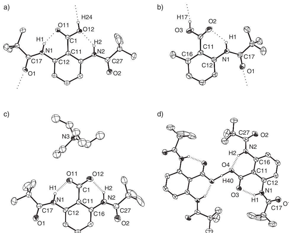
Fig. 1. ORTEP drawings of a) 2,6-( t -BuCONH) 2 C 6 H 3 COOH ( 1 ), b) 2- t -BuCONH-6-MeC 6 H 3 COOH ( 2 ), c) anion part of [NEt 4 ][2,6-( t -BuCONH) 2 C 6 H 3 COO] ( 3 ), and d) [N( n -Pr) 4 ][H{2,6-( t -BuCONH) 2 C 6 H 3 (COO)} 2 ] ( 4 ).
