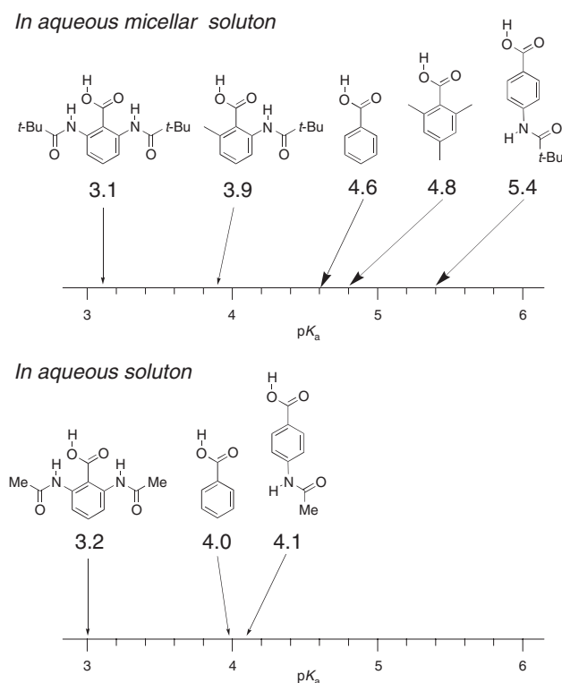
Fig. 4. Summary of pK_a values of series of benzoic acid derivatives.
